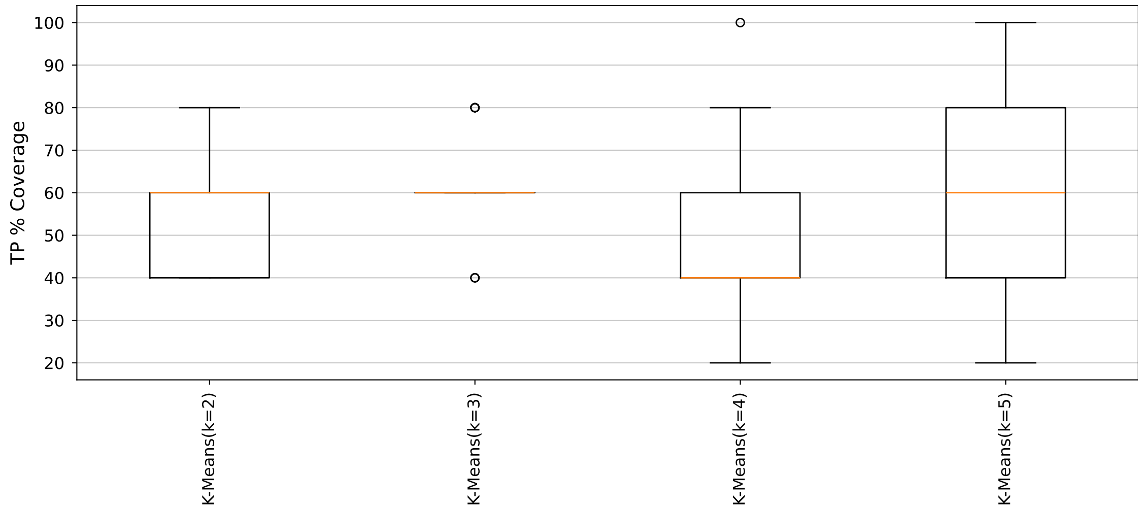
YARA Rules TP Distribution (Cluster42_Size5 dataset)
