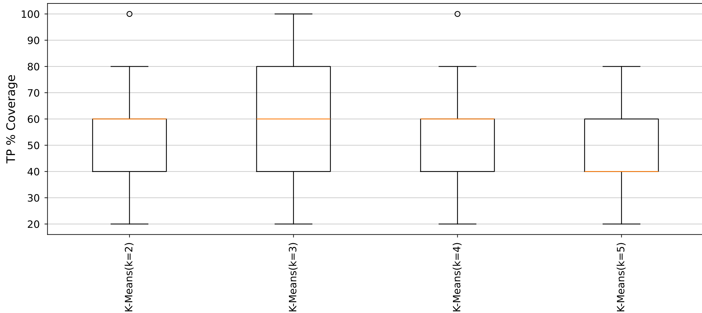
YARA Rules TP Distribution (Cluster43_Size5 dataset)
