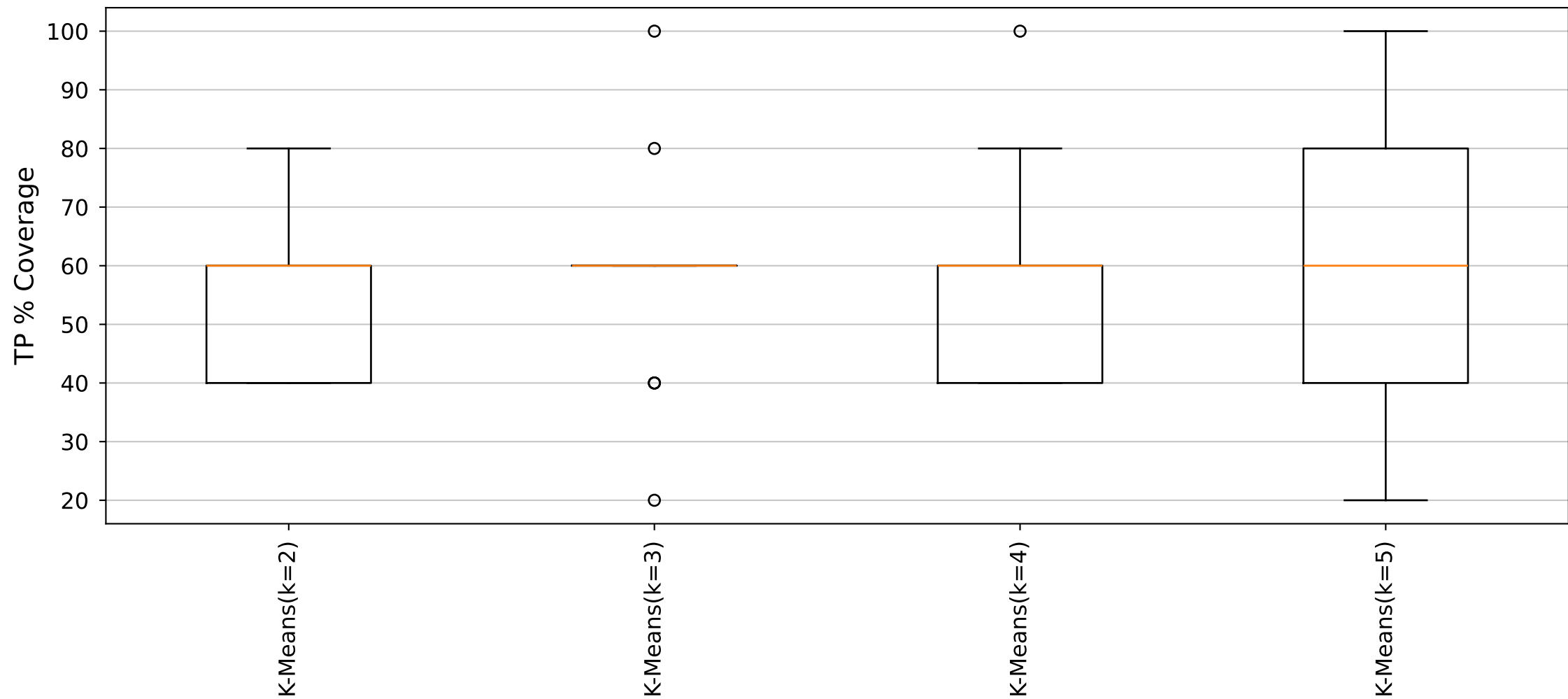
YARA Rules TP Distribution (Cluster45_Size5 dataset)
