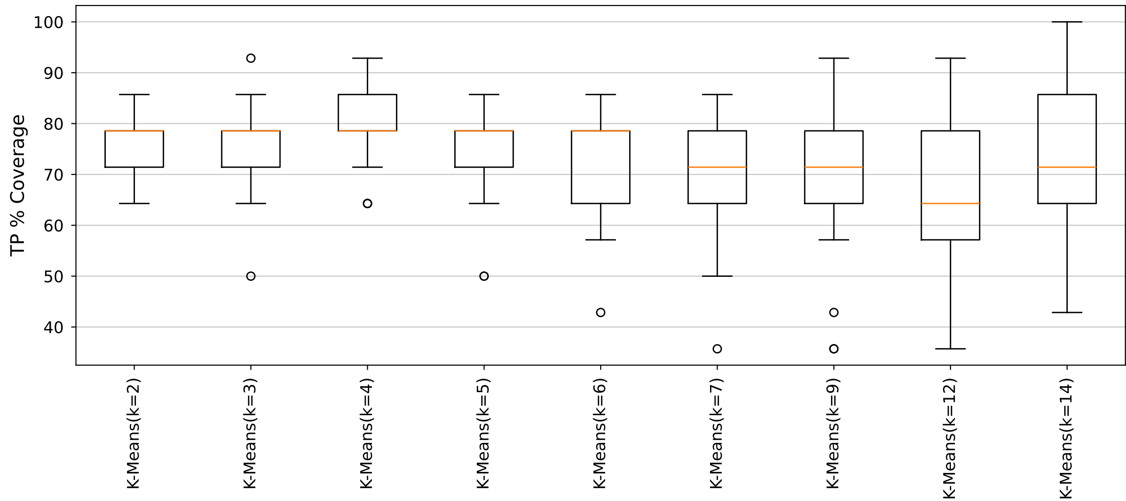
YARA Rules TP Distribution (Cluster7_Size14 dataset)
