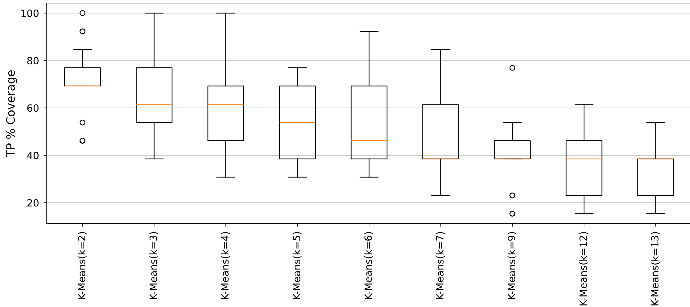
YARA Rules TP Distribution (Cluster8_Size13 dataset)
