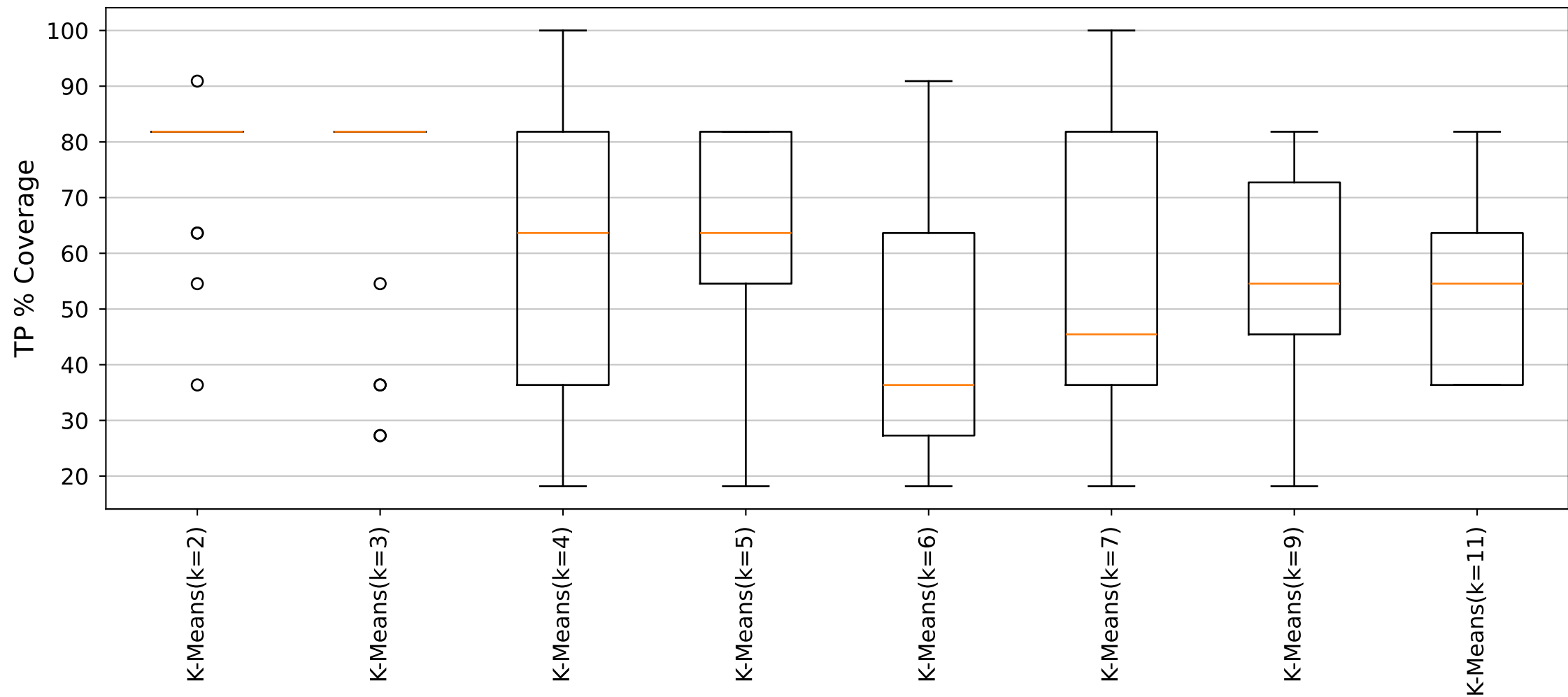
YARA Rules TP Distribution (Cluster9_Size11 dataset)
