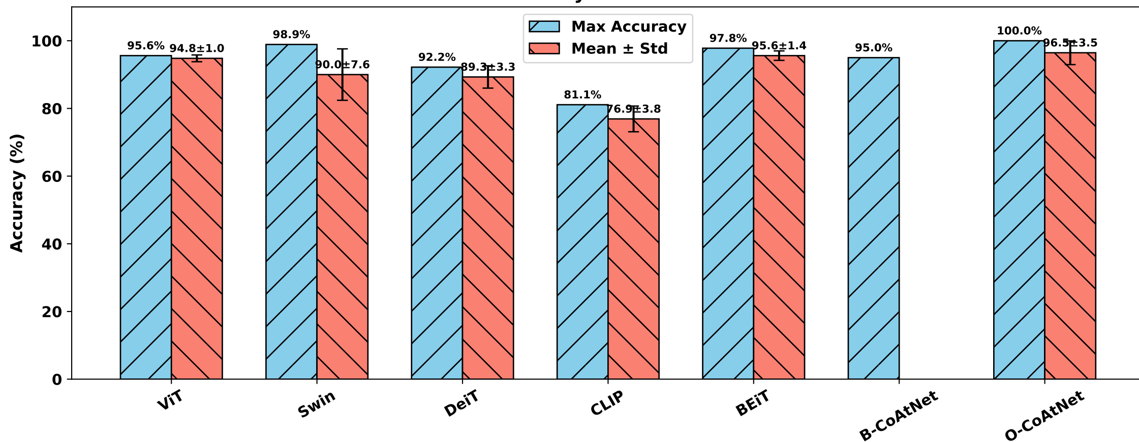
Zoom Dataset: Max Accuracy and Mean \pm Std over 5 Iterations
