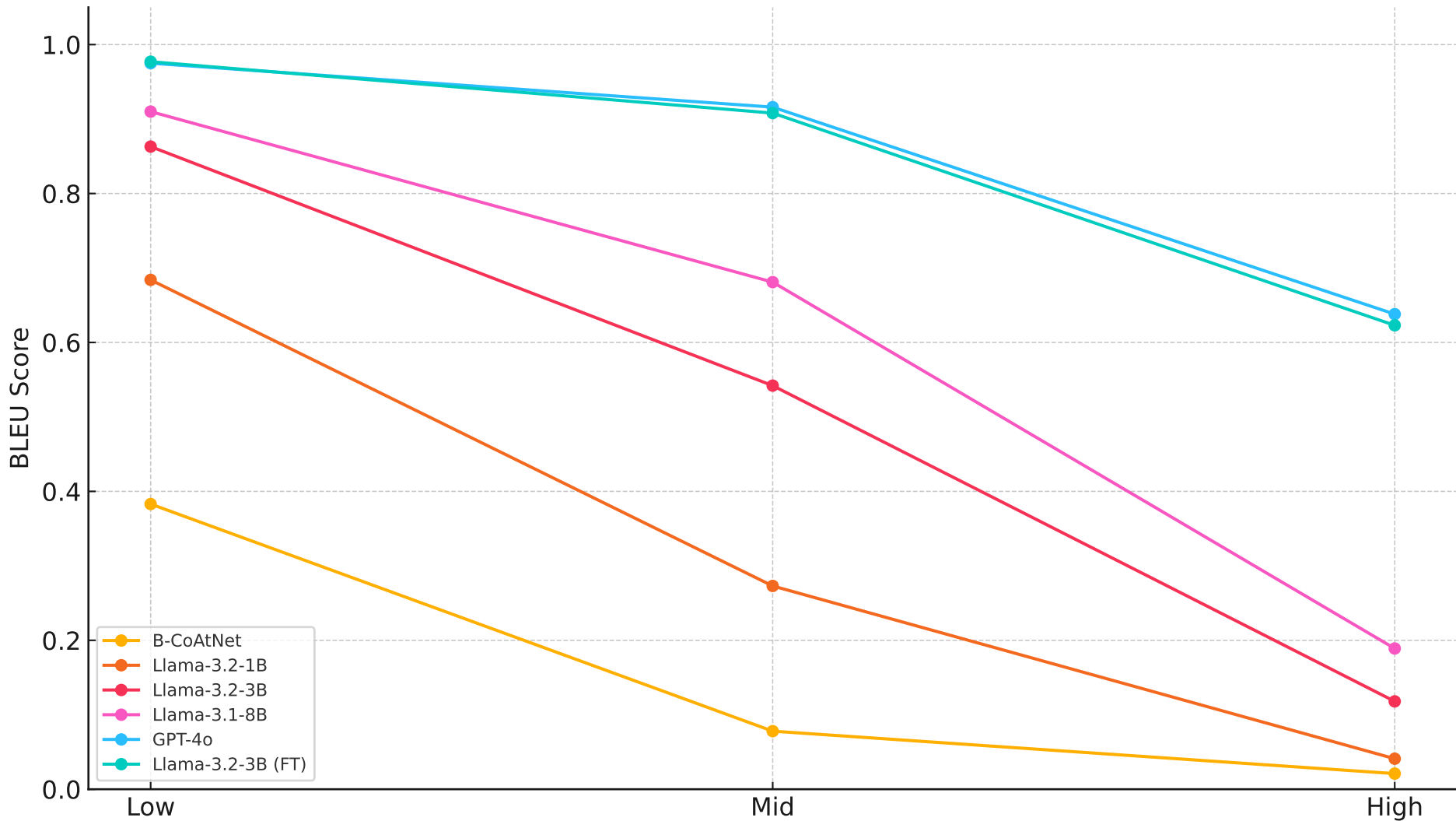
BLEU Score vs. Noise Level (Phone Dataset)
