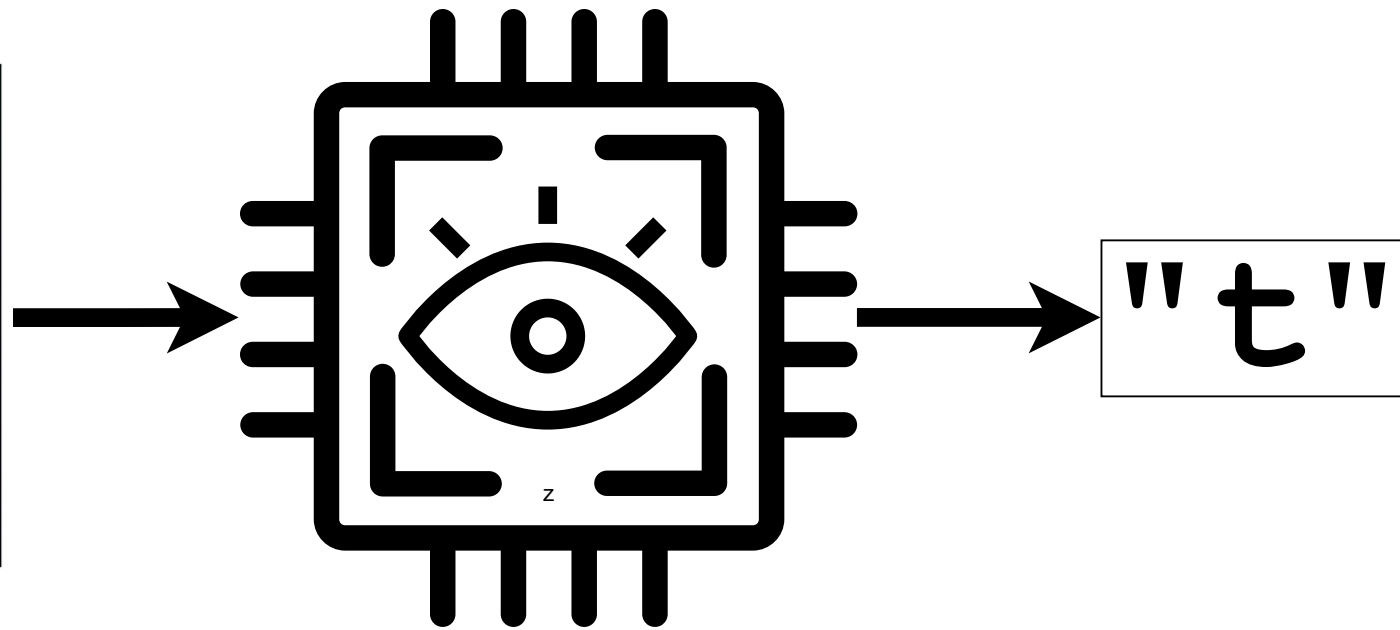
Vision Model
