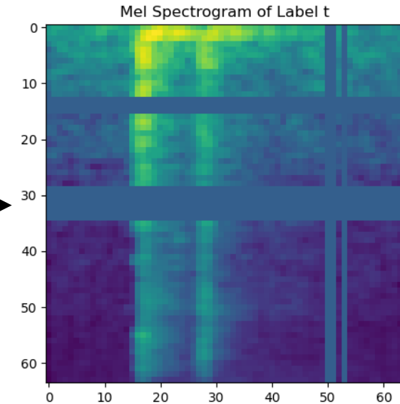
Mel-Spectrogram
