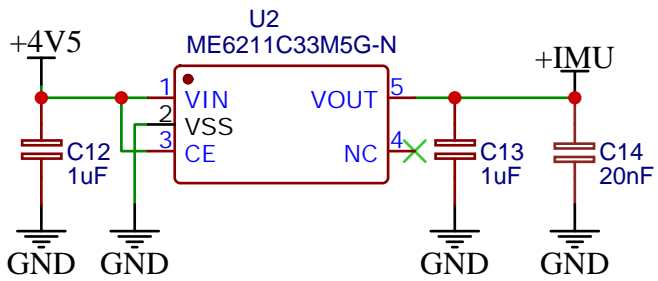
LDO for to IMU
