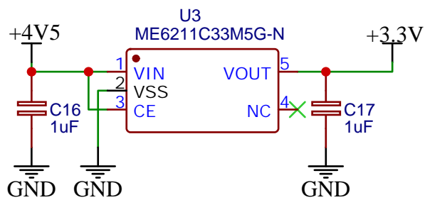
LDO for the STM32
