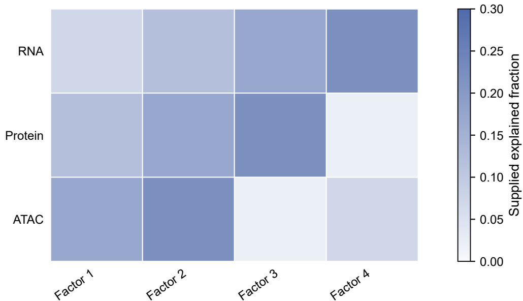
Factor variance by view
