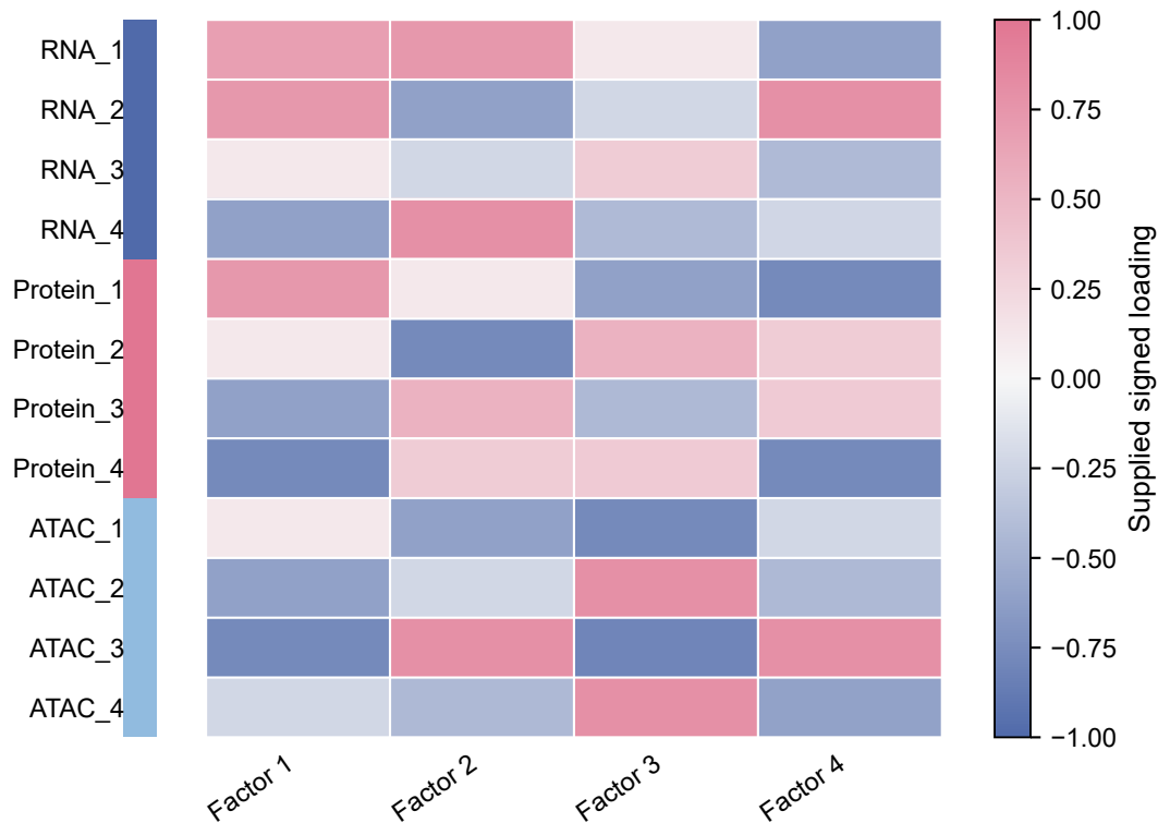
Feature loadings, fixed factor order
