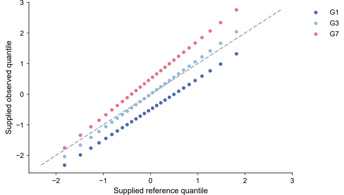
Matched quantiles
