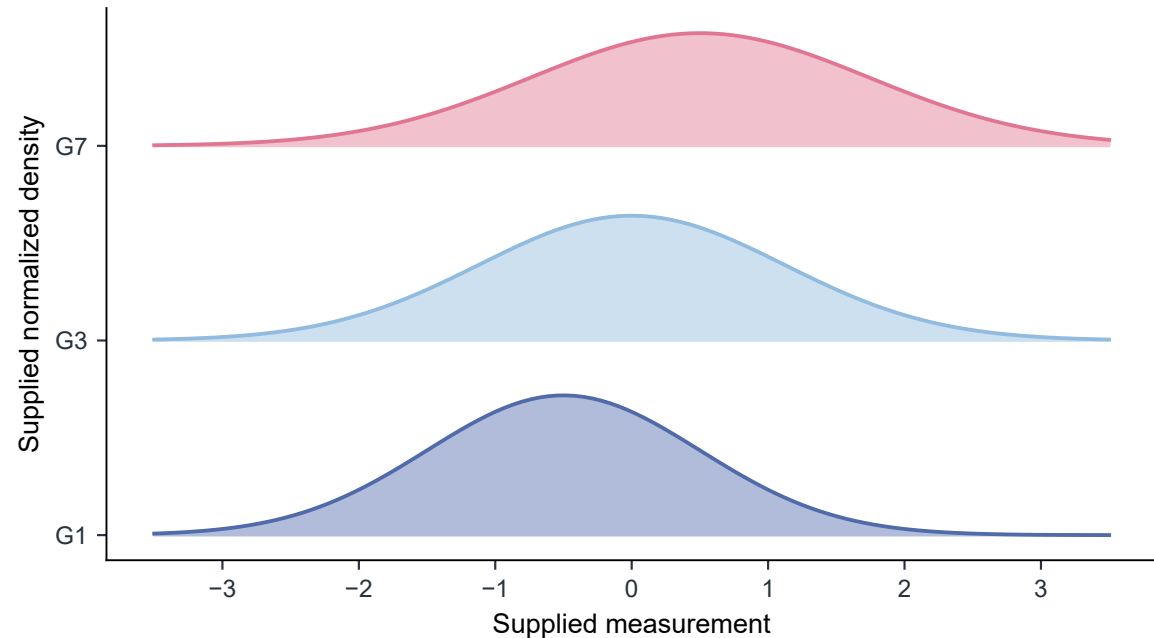
Distribution ridges
