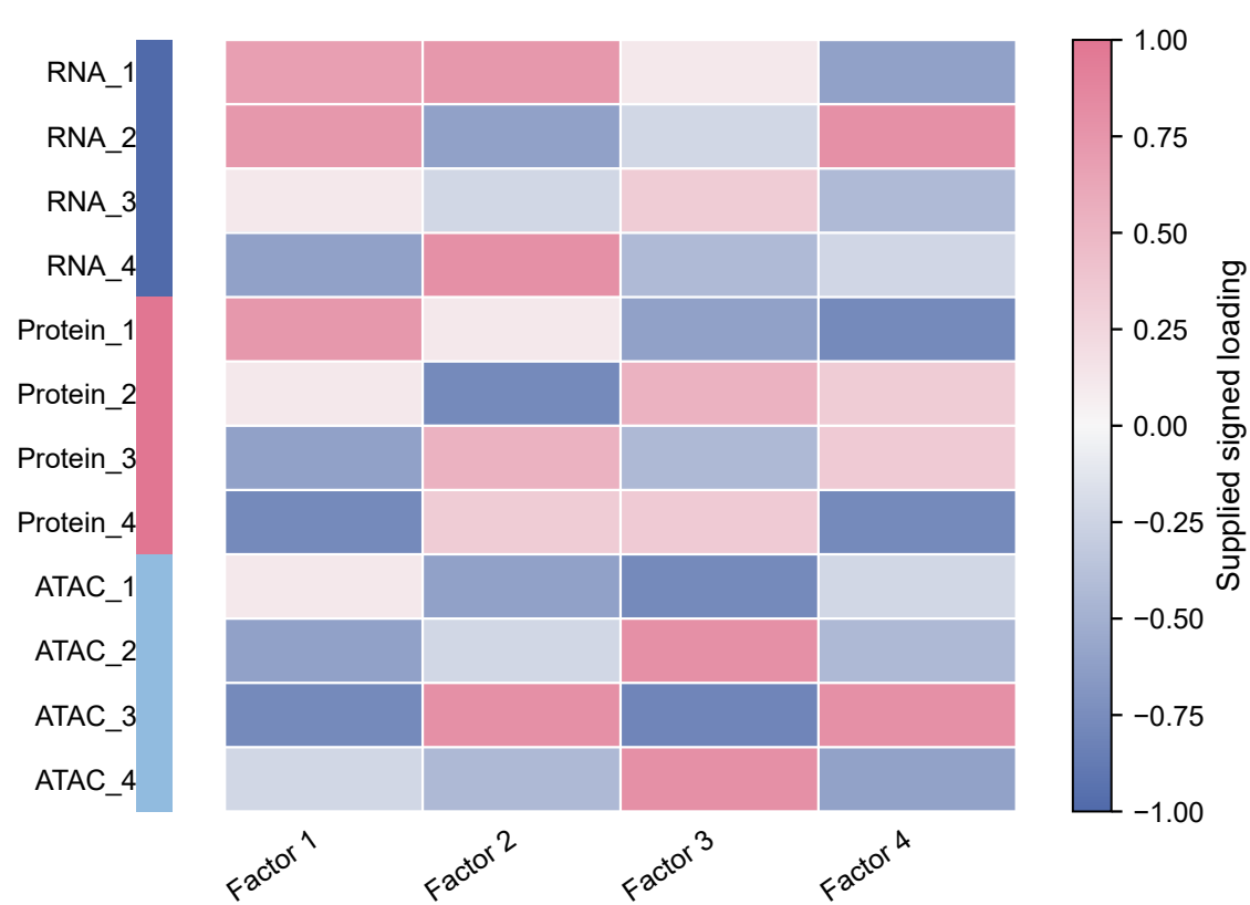
Feature loadings, fixed factor order
