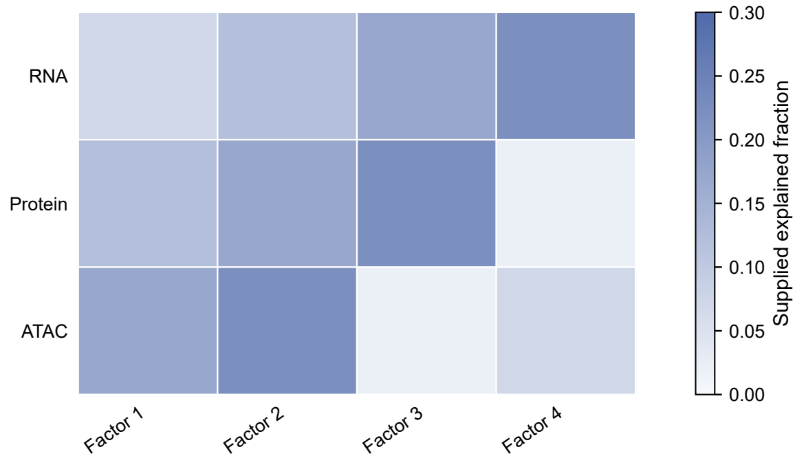
Factor variance by view
