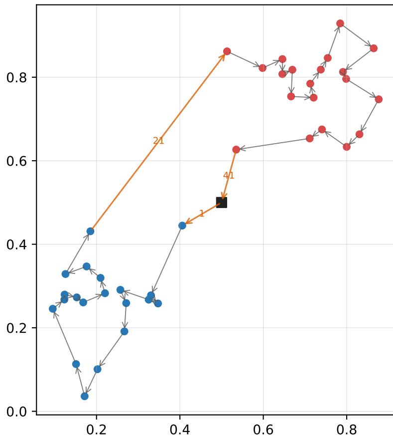
CAADRL, objective 3.2560 inter-cluster switches: 3
