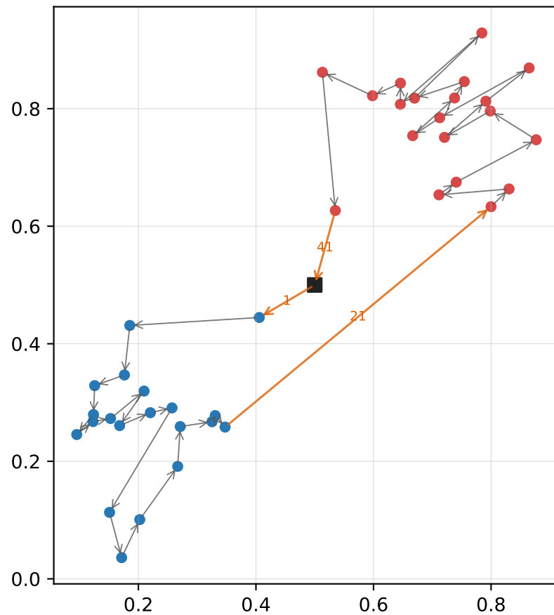
Heter, objective 4.1478 inter-cluster switches: 3
