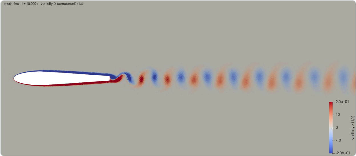
Stage 2, fine mesh, U = 0.2 m/s: the vortex wake that none of the other five tools can show.
