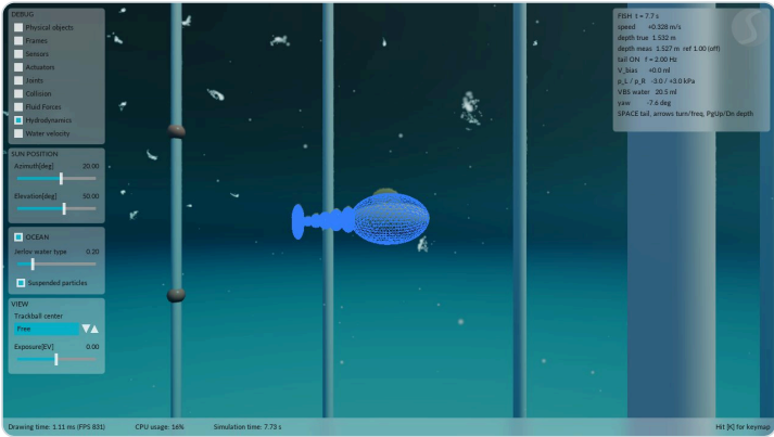
SCREEN Debug view “Hydrodynamics”: the shapes Stonefish uses for buoyancy, drag and added mass, drawn in blue. The status panel (top right) is part of the demo.
