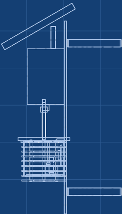
RIGHT VIEW Scale 1:10
