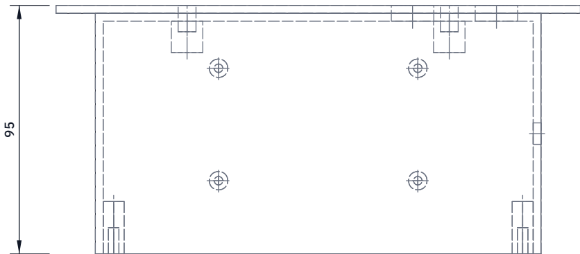
FRONT VIEW Scale 1:2; looking at the front (along +Y)
