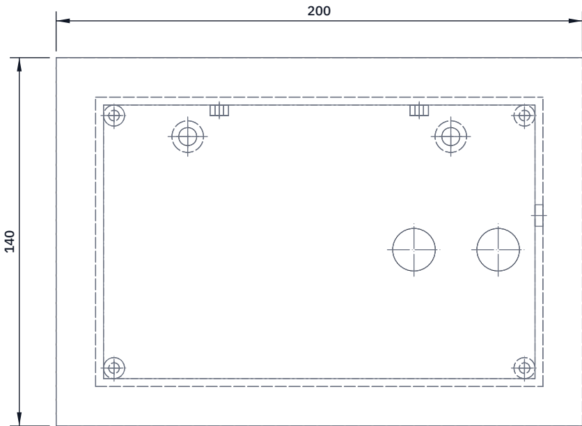
TOP VIEW Scale 1:2; looking down (along -Z)
