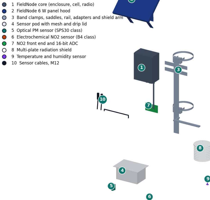
Figure 3. Exploded view with BOM numbers.
