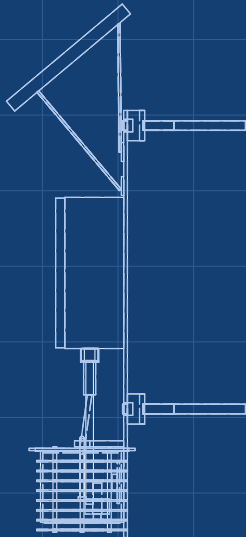
RIGHT VIEW Scale 1:10
