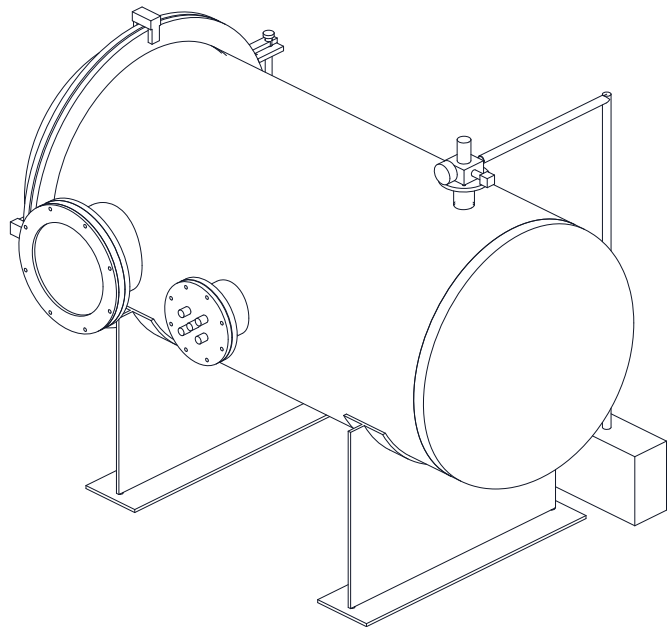
ISOMETRIC VIEW
