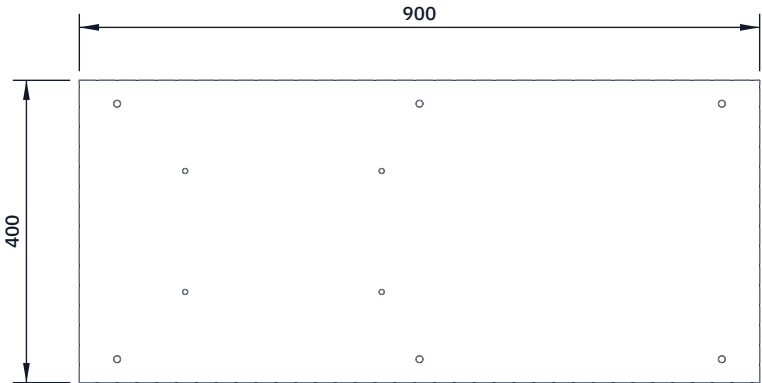
TOP VIEW Scale 1:10; looking down (along -Z)
