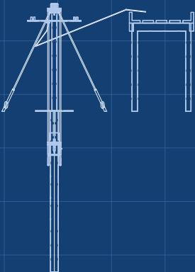
RIGHT VIEW Scale 1:50; looking at the right side (along -X)
