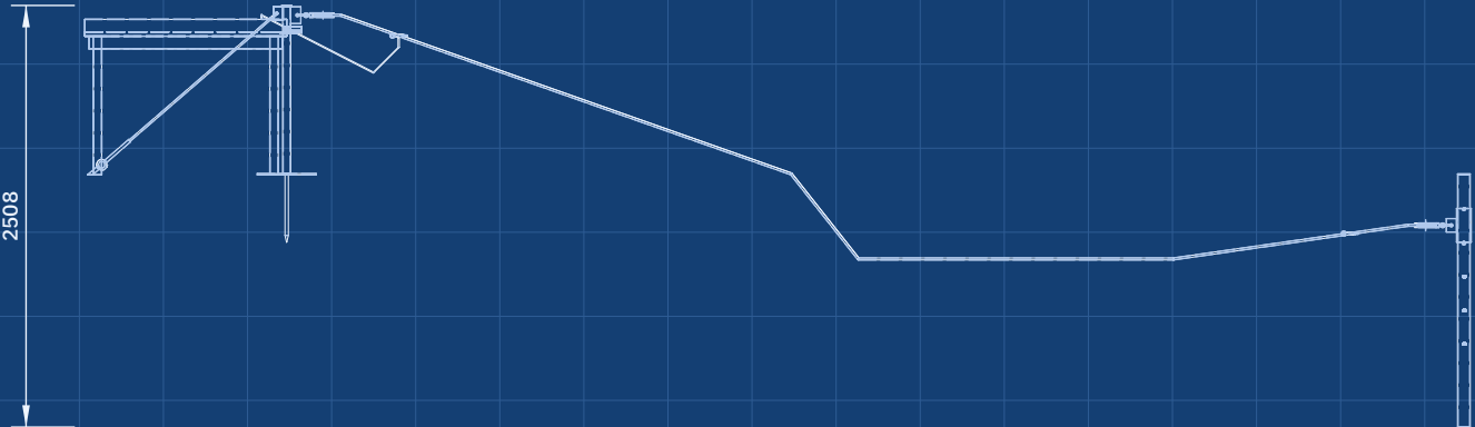
FRONT VIEW Scale 1:50; looking at the front (along +Y)
