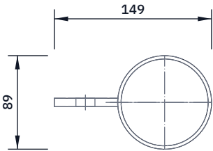
TOP VIEW Scale 1:5; looking down (along -Z)
