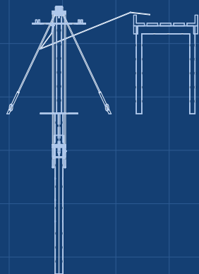
RIGHT VIEW Scale 1:50; looking at the right side (along -X)
