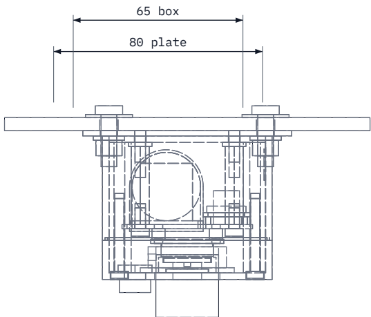
RIGHT VIEW
