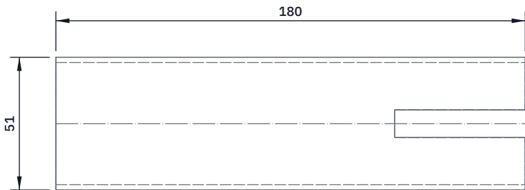
TOP VIEW Scale 1:2; looking down (along -Z)
