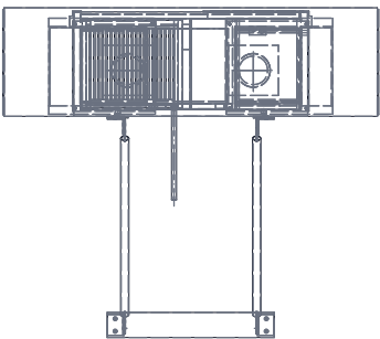
RIGHT VIEW Scale 1:20; looking at the right side (along -X)
