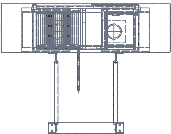
RIGHT VIEW Scale 1:20; looking at the right side (along -X)
