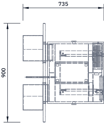
TOP VIEW Scale 1:20; looking down (along -Z)
