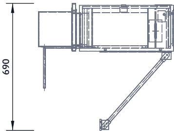
FRONT VIEW Scale 1:20; looking at the front (along +Y)
