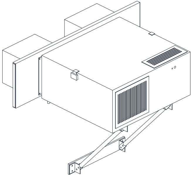
ISOMETRIC VIEW Not to scale; adapter not shown; seen from the front right and above, about 30 deg elevation
