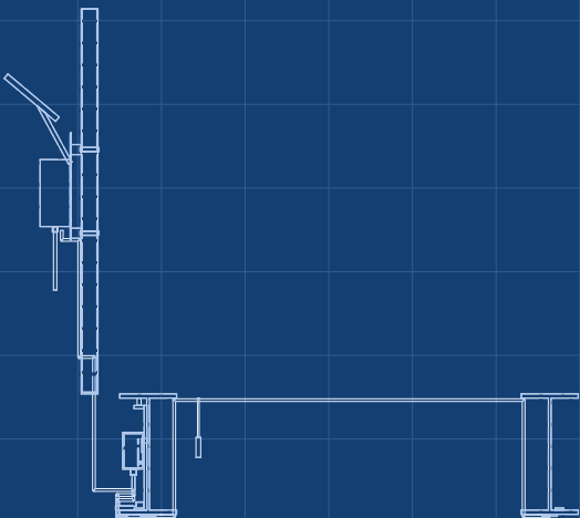
RIGHT VIEW Scale 1:25
