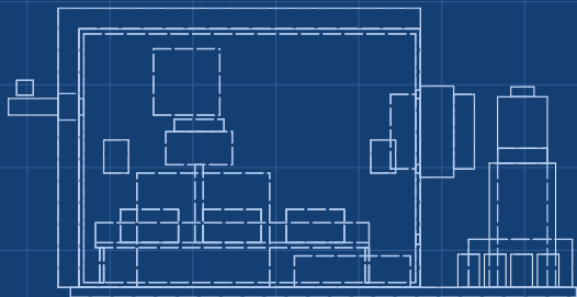
FRONT VIEW Scale 1:10
