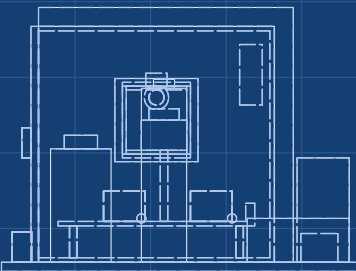
RIGHT VIEW Scale 1:10
