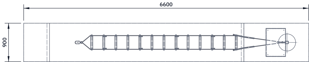
TOP VIEW Scale 1:50; looking down (along -Z)
