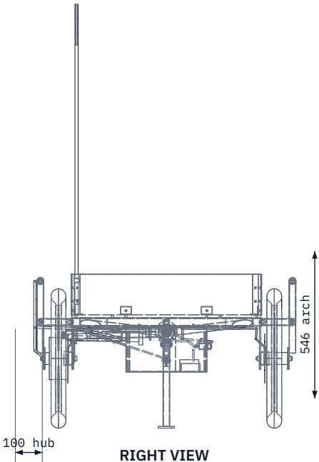
RIGHT VIEW
