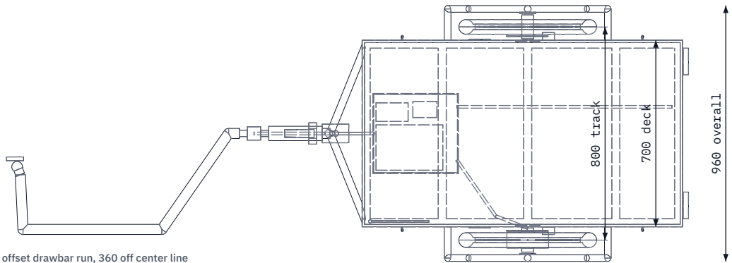
TOP VIEW Scale 1:20
