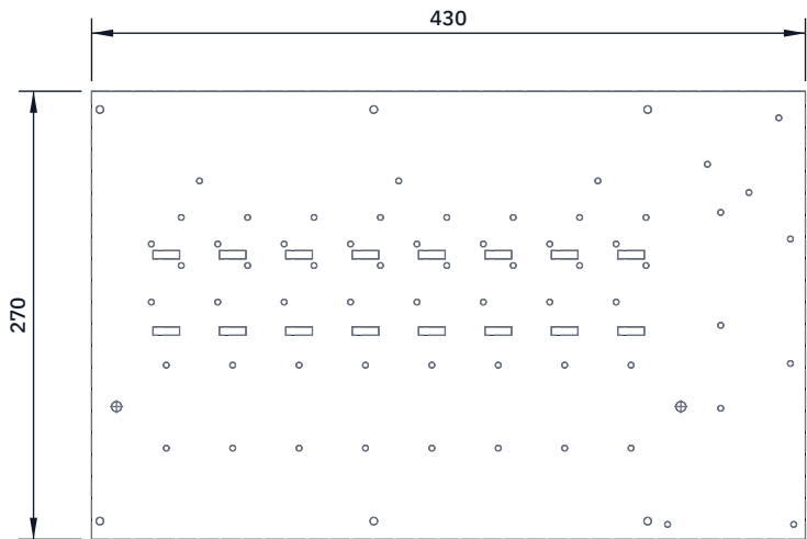
TOP VIEW Scale 1:5; looking down (along -Z)
