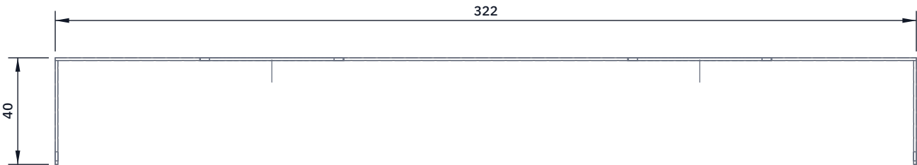
TOP VIEW Scale 1:2; looking down (along -Z)
