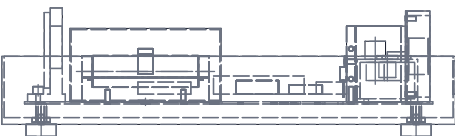
RIGHT VIEW
