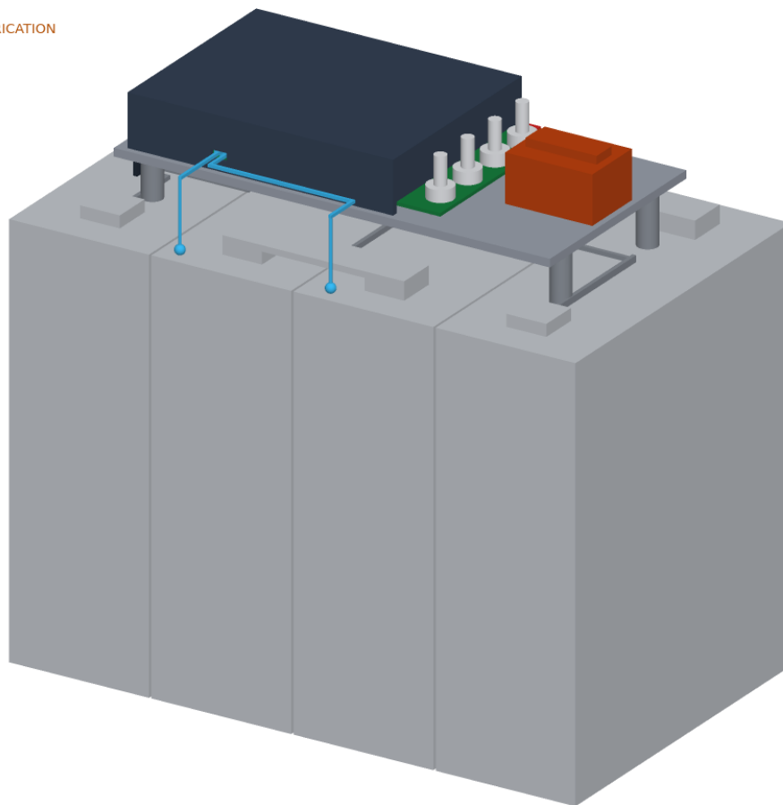
Figure 1. CellGuard on four posts above a 4S LFP pack of 280 Ah prismatic cells, shown for scale. Generated from cad/src/model.py . Concept, not for fabrication.
