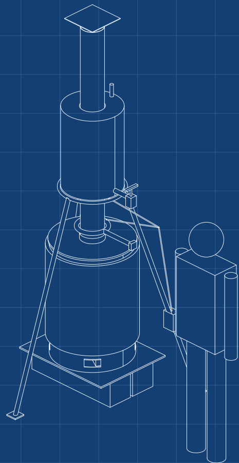
ISOMETRIC VIEW Not to scale; figure is a 1.75 m person
