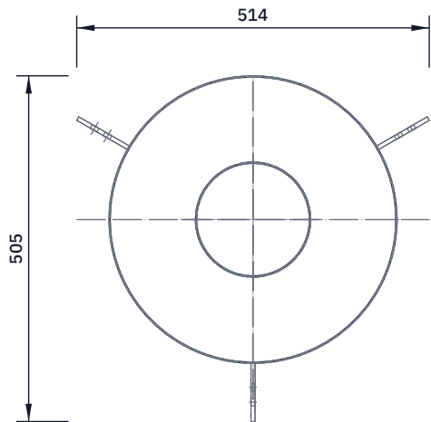
TOP VIEW Scale 1:10; looking down (along -Z)
