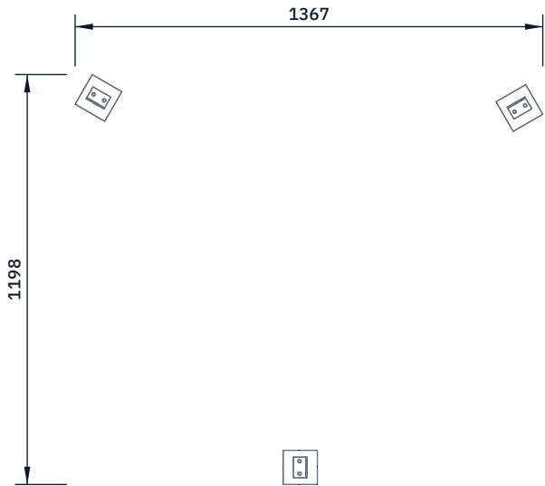
TOP VIEW Scale 1:20; looking down (along -Z)
