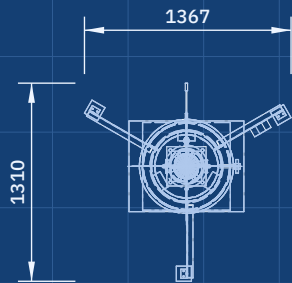
TOP VIEW Scale 1:50; looking down (along -Z)
