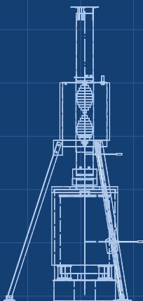
RIGHT VIEW Scale 1:50; looking at the right side (along -X)
