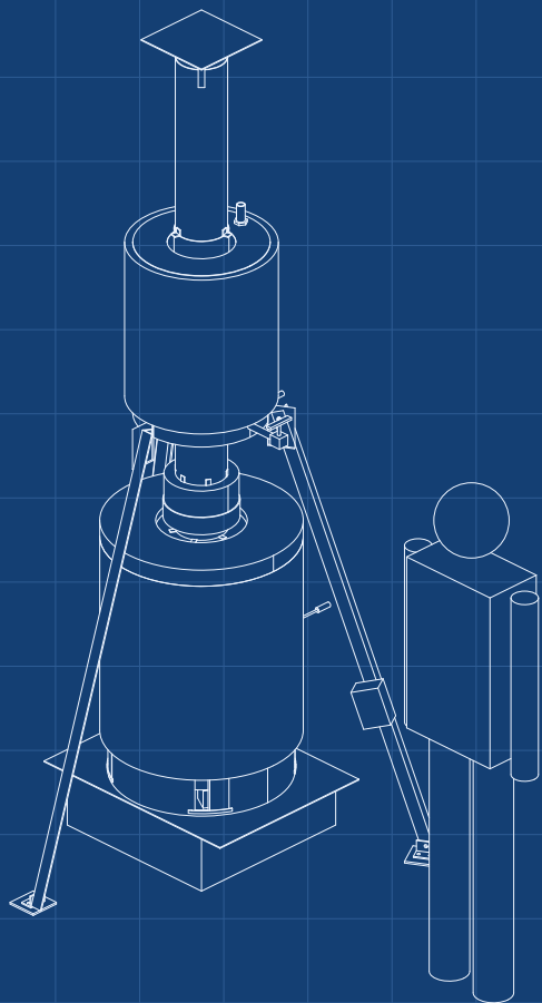
ISOMETRIC VIEW Not to scale; figure is a 1.75 m person; seen from the front right and above, about 30 deg elevation
