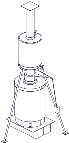
ISOMETRIC VIEW
