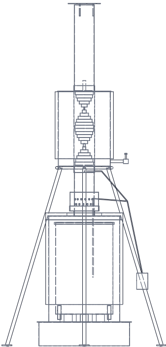
FRONT VIEW Scale 1:30
