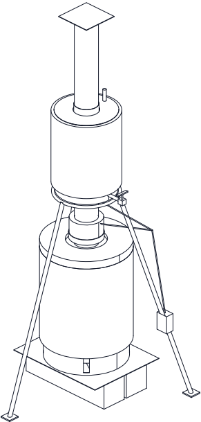
ISOMETRIC VIEW Not to scale
