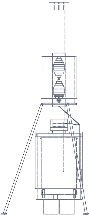
RIGHT VIEW Scale 1:30
