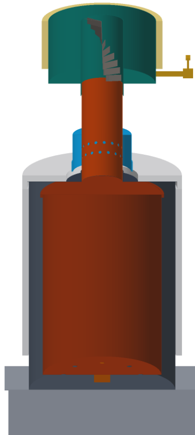
Figure 3. Section looking from the front: retort (3) inside the outer drum (1) with the gas annulus between them, insulation (11, 17) outside and on the lid, lid (2), air shroud (5) and burner throat (6) above, then the blanketed (16) water jacket (8) around its flue sleeve with the spiral baffle (15), and the tap (9). Tripod and logger omitted.
