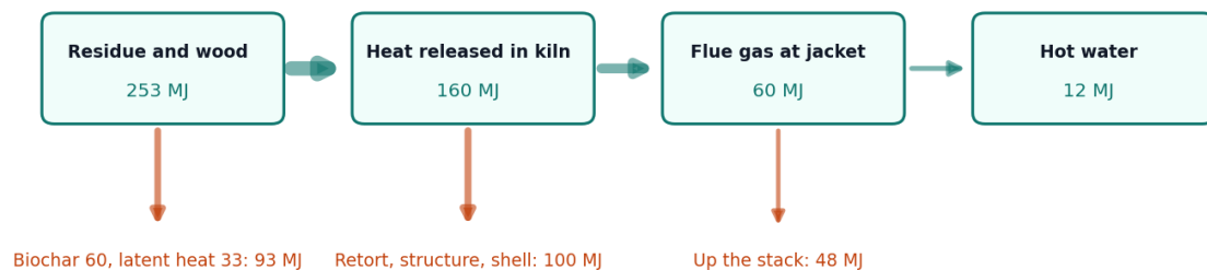
Figure 2. Energy per batch, central estimates from CCB-CAL-001 v0.2: 12.0 kg of residue at 16.0 MJ/kg (air-dry, higher heating value) plus 3.7 kg of wood at 16.2 MJ/kg (lower heating value); 2.96 kg of char at 20.2 MJ/kg; with the baffle and jacket blanket the jacket takes about 19 % of the flue gas heat.
