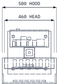
TOP VIEW Scale 1:20
