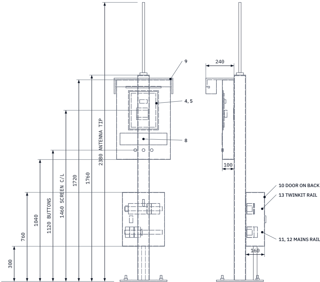
FRONT VIEW Scale 1:20
