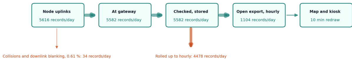
Figure 2. LoRaWAN data flow for the reference neighborhood, in records per day (CTW-CAL-001): 0.61 % lost to collisions and downlink blanking, and 5,582 stored records rolled up to 1,104 hourly records for the open export. PotholeLog and DockHub rows, pulled from their operators, are not shown.
