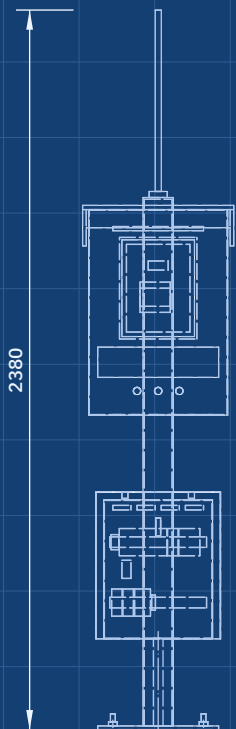
FRONT VIEW
