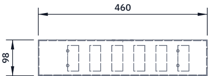
TOP VIEW Scale 1:10; looking down (along -Z)
